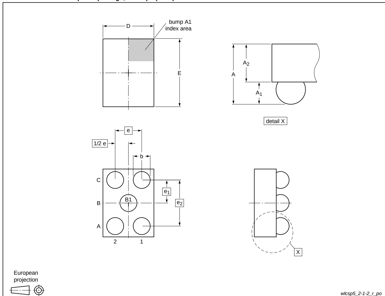
Fig 1. Package outline IP4059CX5/LF (WLCSP5)
